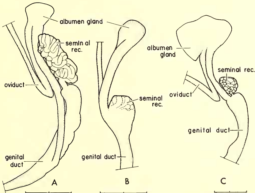
TEXT-FIG. 10. Posterior view of terminal segments of the genital ducts and associated structures in three species of Amphicyclotus . A. A. paulsonorum new species, toptype. B. A. parvus Thompson, paratype. C. A. t. spiralis new subspecies, toptype. Scales equal 2 mm.
